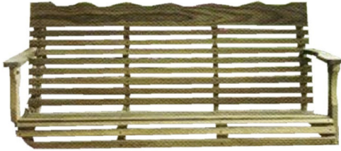
WW-2010 Swing -- 4' 52 1/4"w x 27"d x 24"h Wt. 41 lbs.
